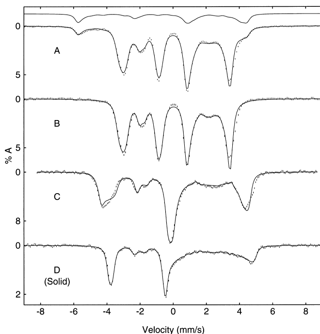
Fig. 5. Mössbauer spectra of ^{57}\text{Fe} -enriched 3 dissolved in ethanol (a)–(c) and polycrystalline 3 (d). The spectra in (a) and (b) were recorded in a parallel applied field of 0.05 T at 4.2 K (a) and 1.5 K (b). (c) Spectrum recorded at 4.2 K in an 6.0 T field applied parallel to the observed \gamma -radiation. The solid lines are theoretical curves generated from Eqs. (1) and (2) with the parameter set listed in Table 1. The solid line drawn above the 4.2 K low field spectrum (a) shows the contribution of the upper Kramers doublet of the S=3/2 system. The spectrum of polycrystalline 3 (d) was recorded at 4.2 K in a parallel applied field of 6.0 T.
