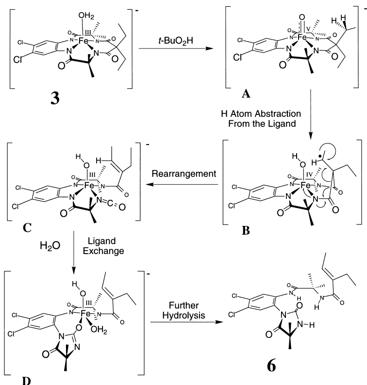
Scheme 2. Proposed ligand oxidative degradation scheme. In the scheme, we have drawn an \text{Fe}^{\text{V}}\text{-oxo} intermediate, A . With this, we do not wish to imply any specific allocation of oxidizing equivalents to the metal or the ligand. Alternative formulations include an \text{Fe}^{\text{IV}}\text{-oxo} /ligand radical cation. In addition, the abstracting entity could be a free radical.
