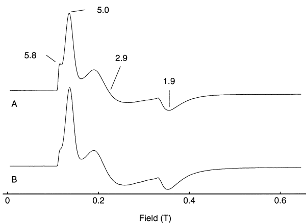
Fig. 4. Low temperature EPR spectra of complex 3 dissolved in ethanol recorded at T=20 K (upper trace) and T=4 K. Spectra were recorded at 9.46 GHz at a microwave power of 80 mW (upper trace) and 0.5 mW (lower).
