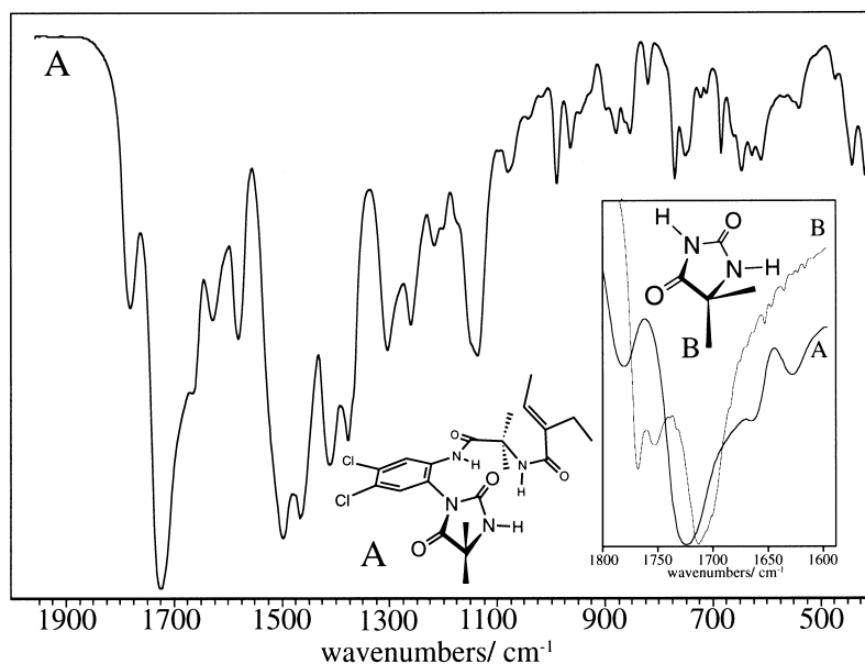
Fig. 11. The IR spectrum of solid 6 showing the strong 1723 cm -1 band. Insert: comparison of the 1600–1800 cm -1 region of 6 [ A ] and the parent dimethylhydantoin heterocycle [ B ].
