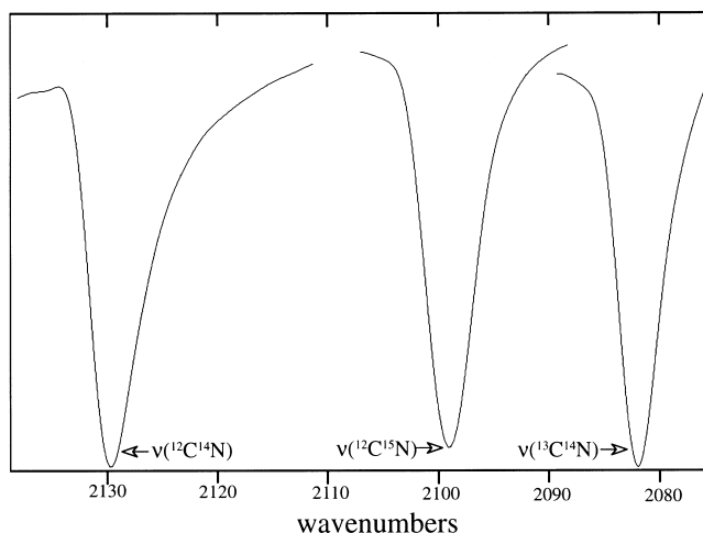
Fig. 8. IR spectra showing the \nu(\text{CN}) region for [\text{PPh}_4]\mathbf{5} with ^{12}\text{C}^{14}\text{N}^- , ^{12}\text{C}^{15}\text{N}^- , and ^{13}\text{C}^{14}\text{N}^- ligands.
