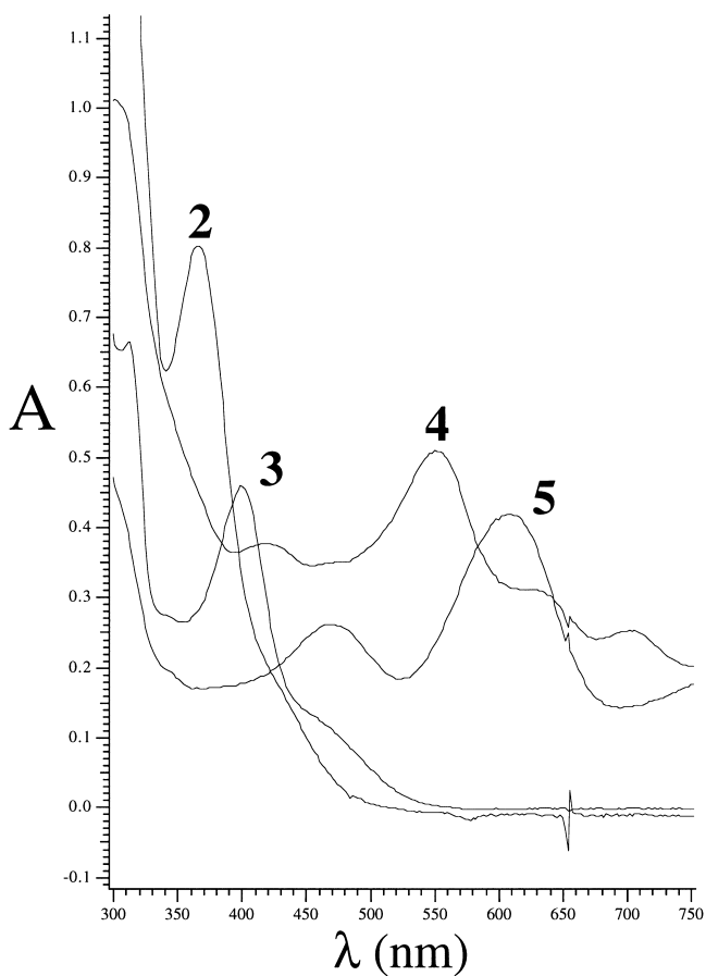
Fig. 1. UV-vis spectra in \text{CH}_3\text{CN} of 2 , 3 , 4 and 5 . Complex, Concentration (M), \lambda_{\text{max}} (nm), \epsilon : 2 1.48 \times 10^{-4} 365, 5410; 3 5.51 \times 10^{-5} 400, 8320; 4 1.05 \times 10^{-4} 533, 5160; 5 4.16 \times 10^{-5} 471, 6270–609, 10 050.
